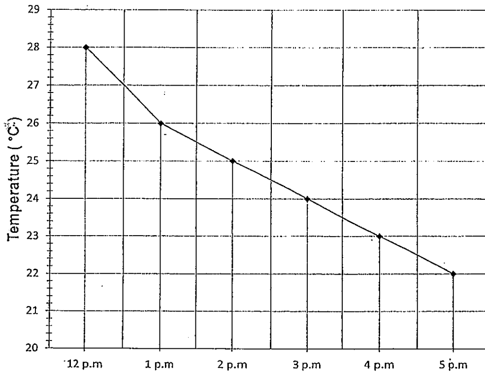
Daily Temperature
